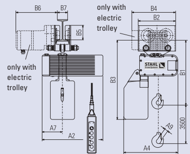
Chain hoist with trolley
